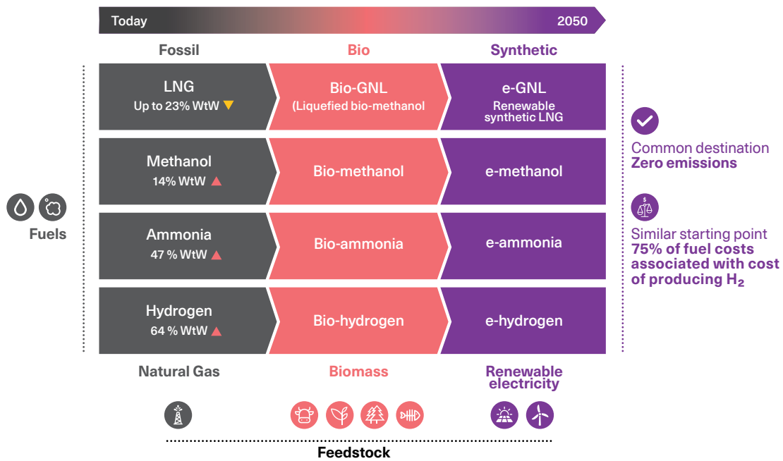
Figure 5.1 Alternative paths for the decarbonization of maritime transport
